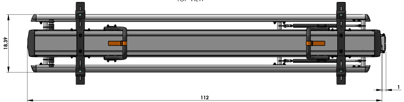
TOP VIEW
