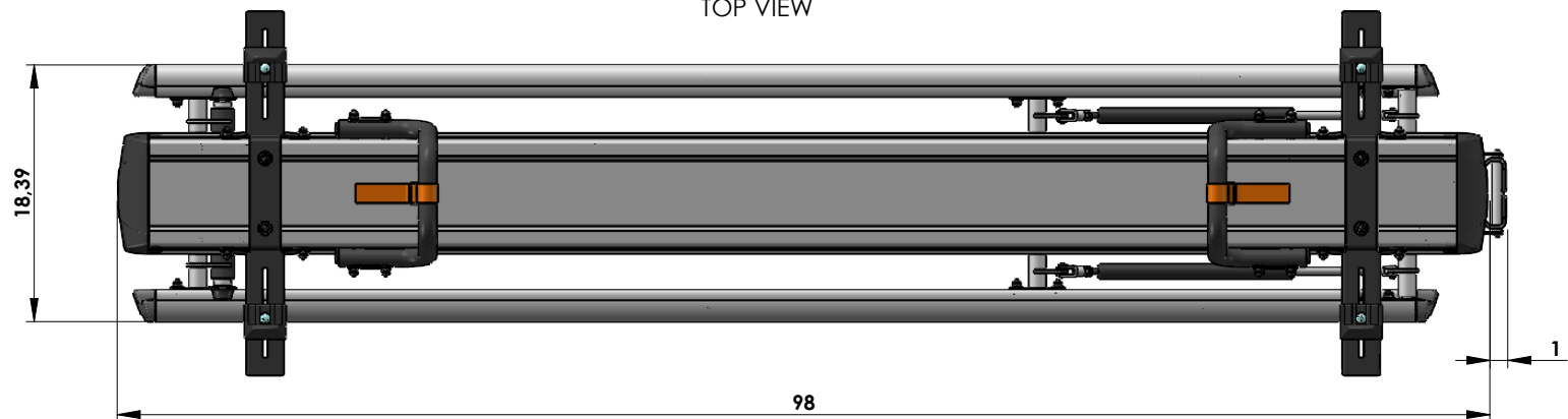
TOP VIEW
